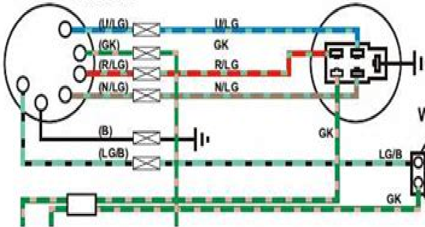
† WIPER/WASHER SWITCH
