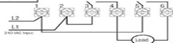
Timer Power
