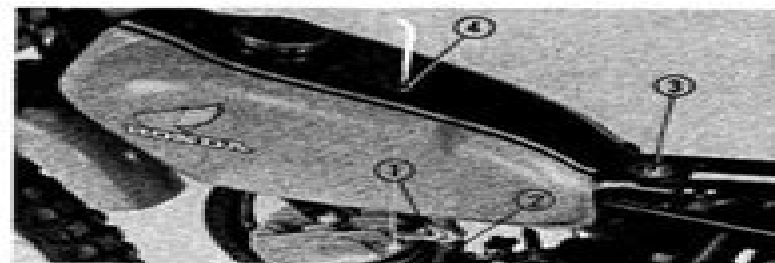
Fig. 4-50 (1) Fuel valve (3) Bolt (2) Fuel hose (4) Fuel tank
