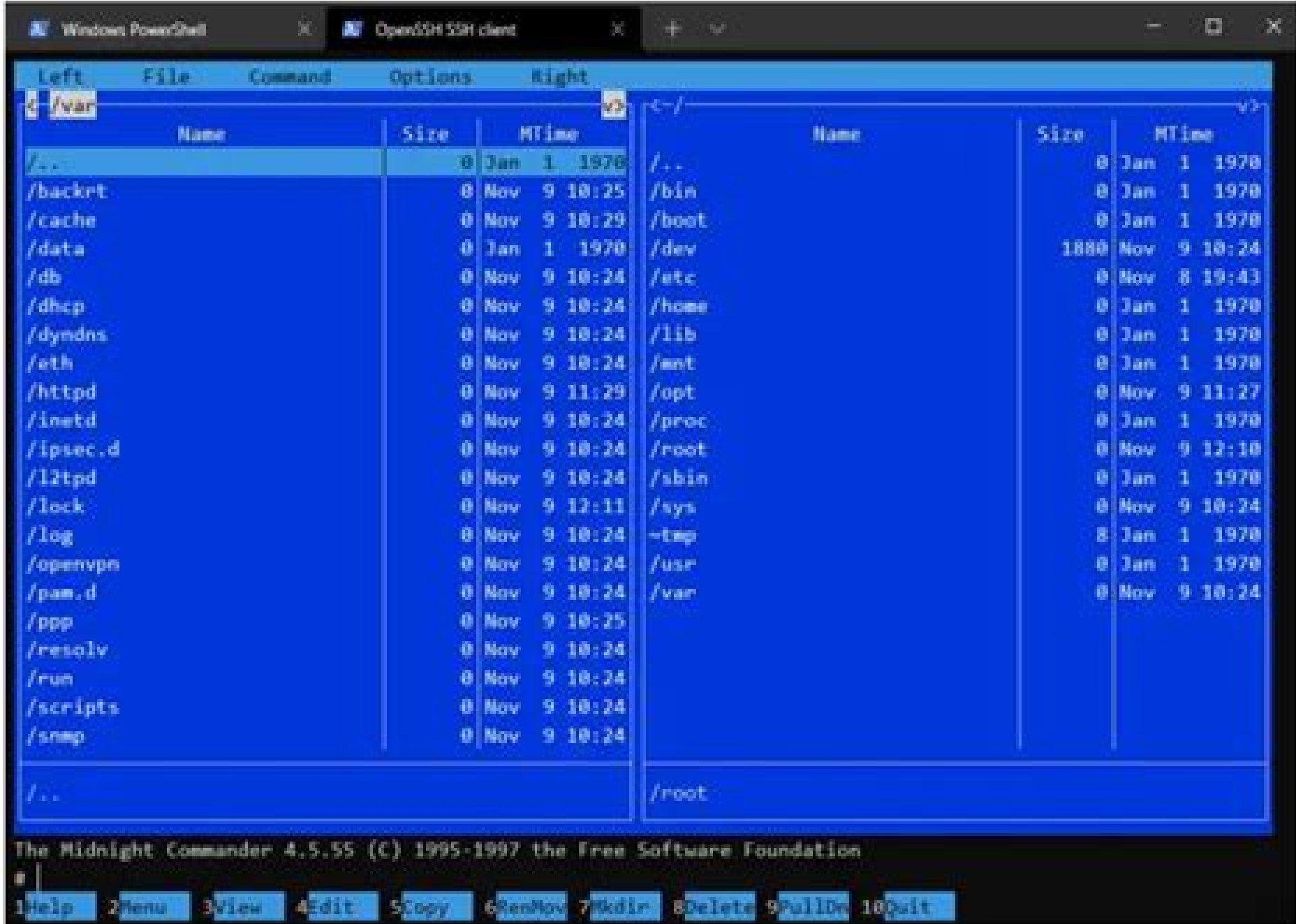
Figure 1: Midnight Commander
