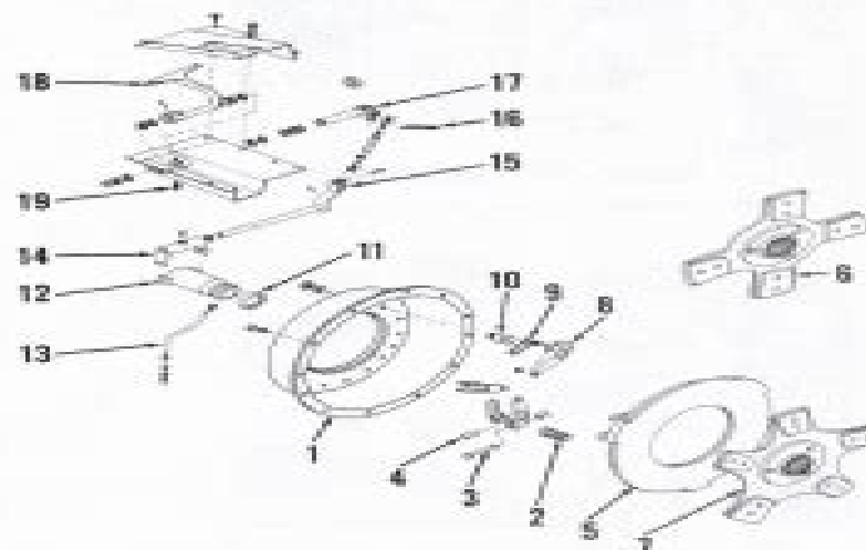
Fig. 198—Exploded view of clutch and linkage. Disc (6) with four pads is used with brown springs (2) on MP 1105 models only.
