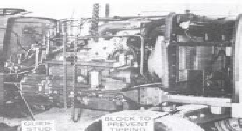
Fig. 197—View showing supports necessary when splitting. 3/4 in. cylinder model is shown but blocking is similar for MP 1135.
