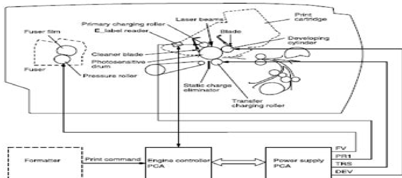
Figure 18. Image-formation system
