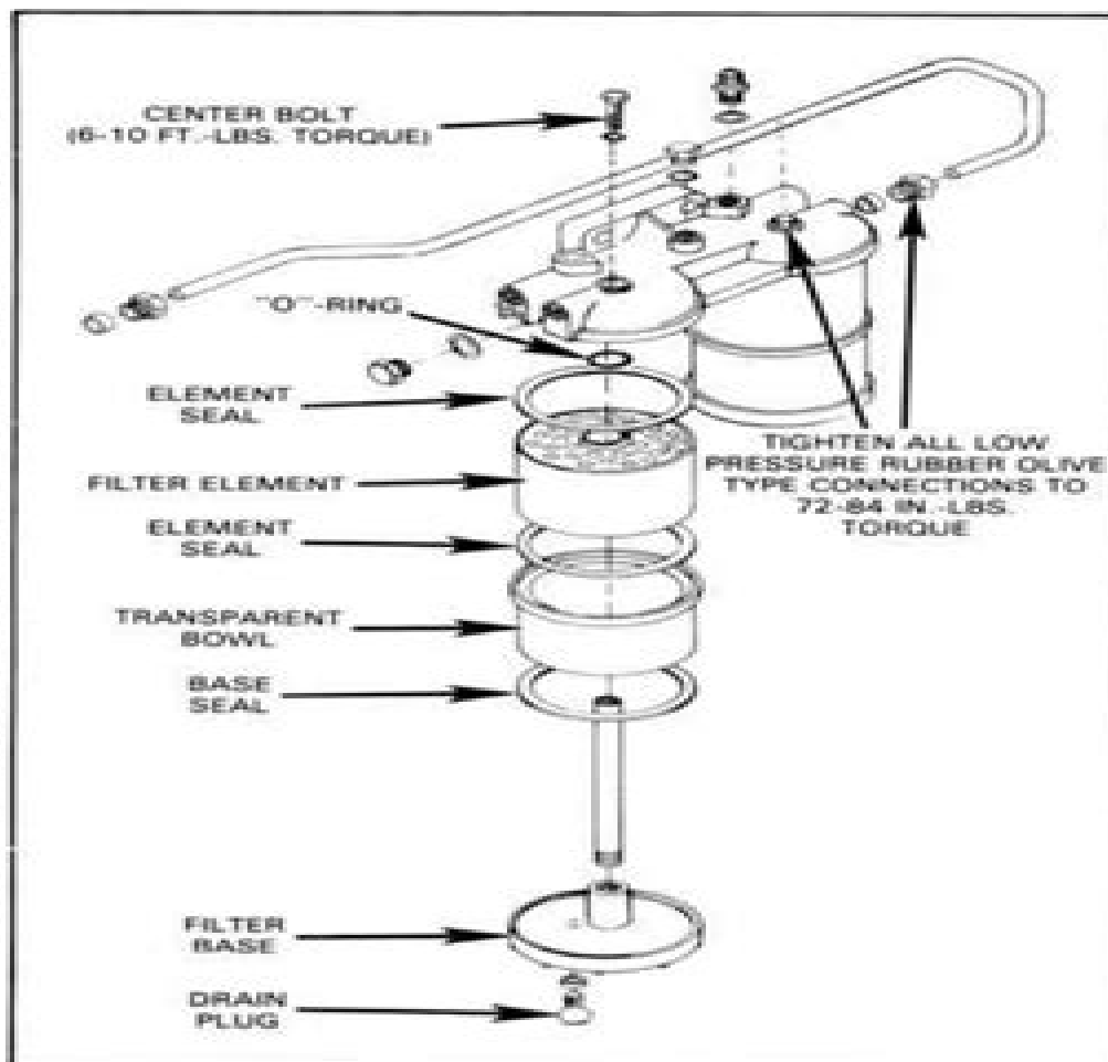
FIG. 20 — FUEL FILTER — IDENTIFICATION AND SEQUENCE OF PARTS
