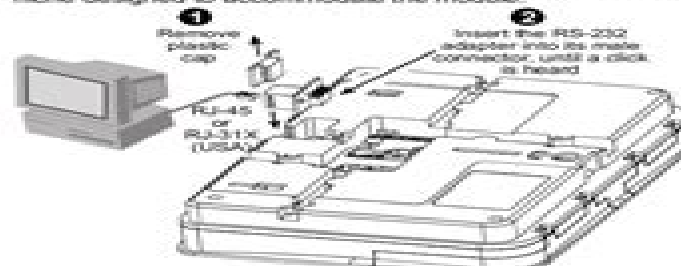
Figure 3.4 - Connecting the PowerMax+ to a Computer
