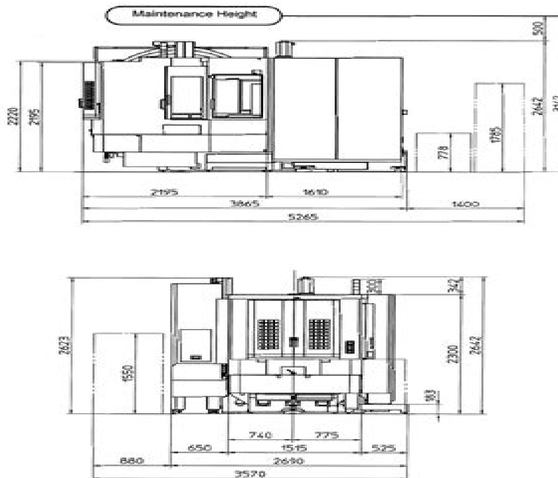
Figure 2.3 Side and Front View of Machine (Tool Magazine A99 and Left-Discharge Conveyor Specs.)
