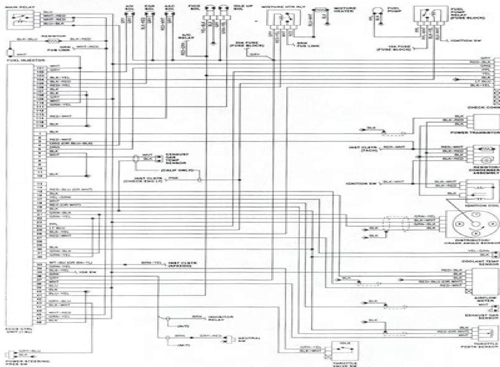
Fig. 45: 1989-90 Sentra & Pulsar NX 1.6L Fuel Injection Wiring Diagram (1989-90 Sentra Shown, 1989-90 Pulsar NX Similar)
