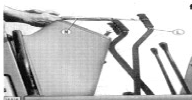
Checking clutch engagement force (engine off). L. Clutch lever - M. Spring scale.
