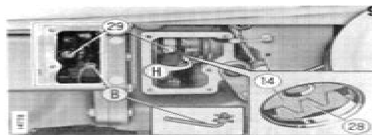
Adjusting clutch engagement. B. Wrench 290954 - H. Aperture - 14. Retainer - 28. Lock ring - 29. Reference screw.
