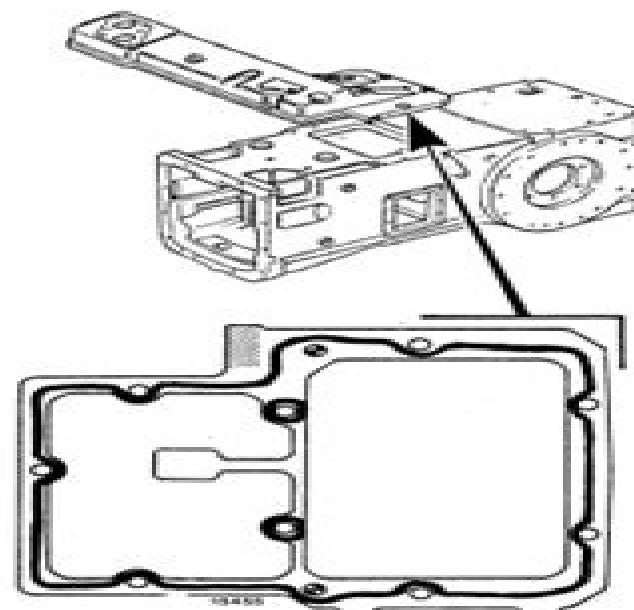
Applying jointing compound for relay lever support cover installation on rear transmission housing. Jointing compound types are indicated on page 6, section A.
