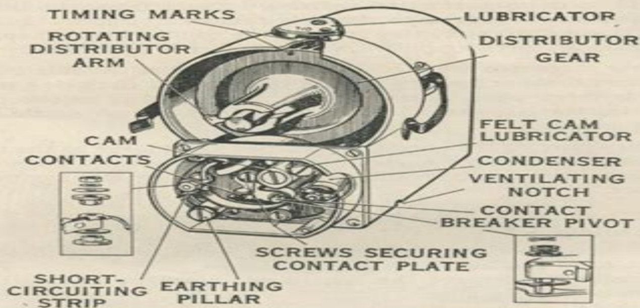
Fig. 2. Model RF4 Magneto with Distributor Block and Contact Breaker Cover removed. The inset sketches show order of assembly of Contact Breaker Terminal and Pivot Components.
