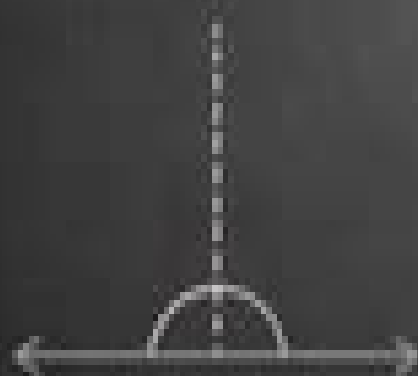
straight angle
