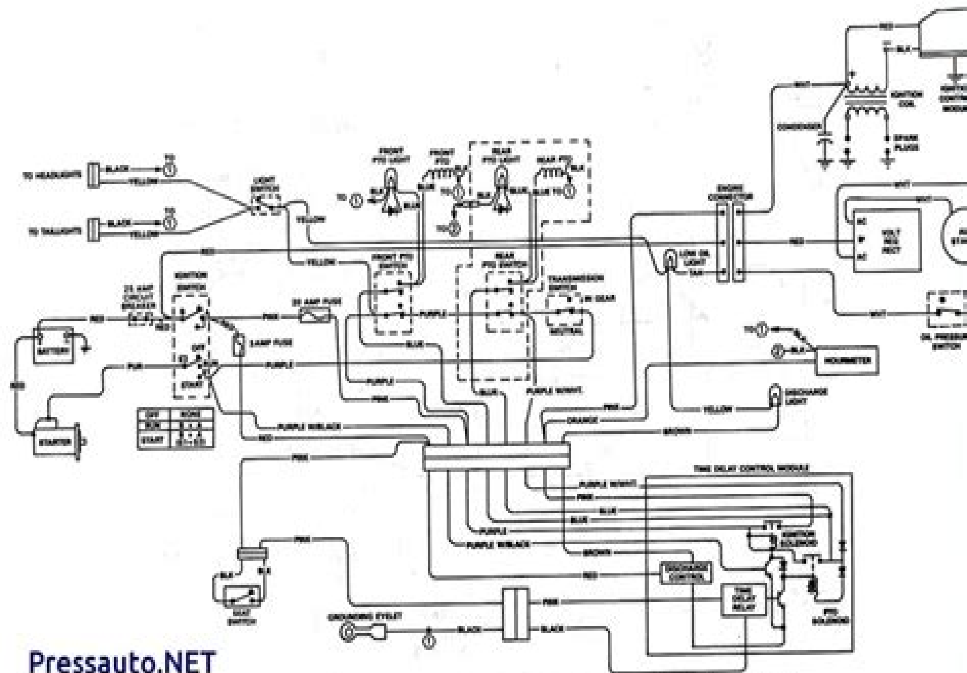
Fig. JD23—Wiring diagram for Models 318 and 420 after serial number 475,001.
