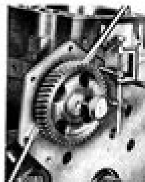
Fig. 10 - Measuring Camshaft End Play
