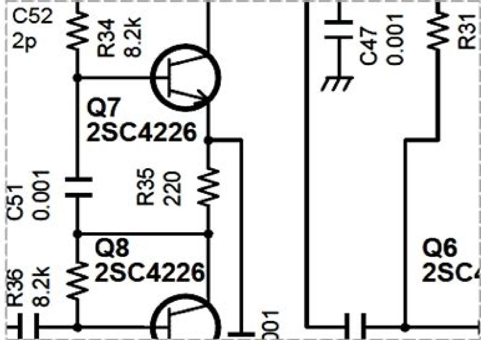
Preview: ICOM IC-F310 /F320 schematic diagram
