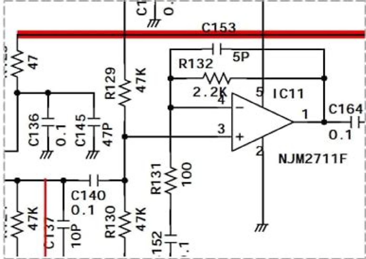
Preview: ICOM UR-FR6000 schematic diagram
