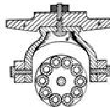
FIG. 5. SECTION THROUGH BARREL, BREECH AND MUZZLE ENDS INDICATED.
