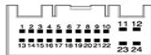
Connector B
