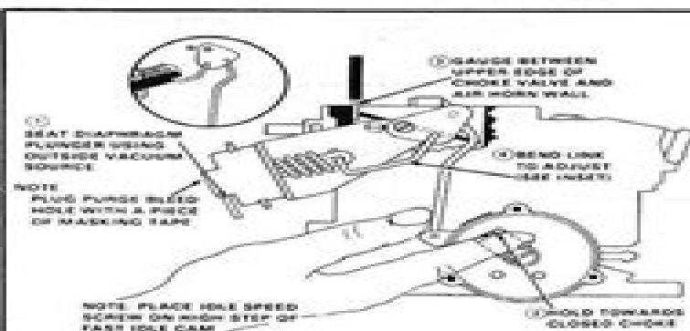
VACUUM BREAK ADJUSTMENT FIG. 25
