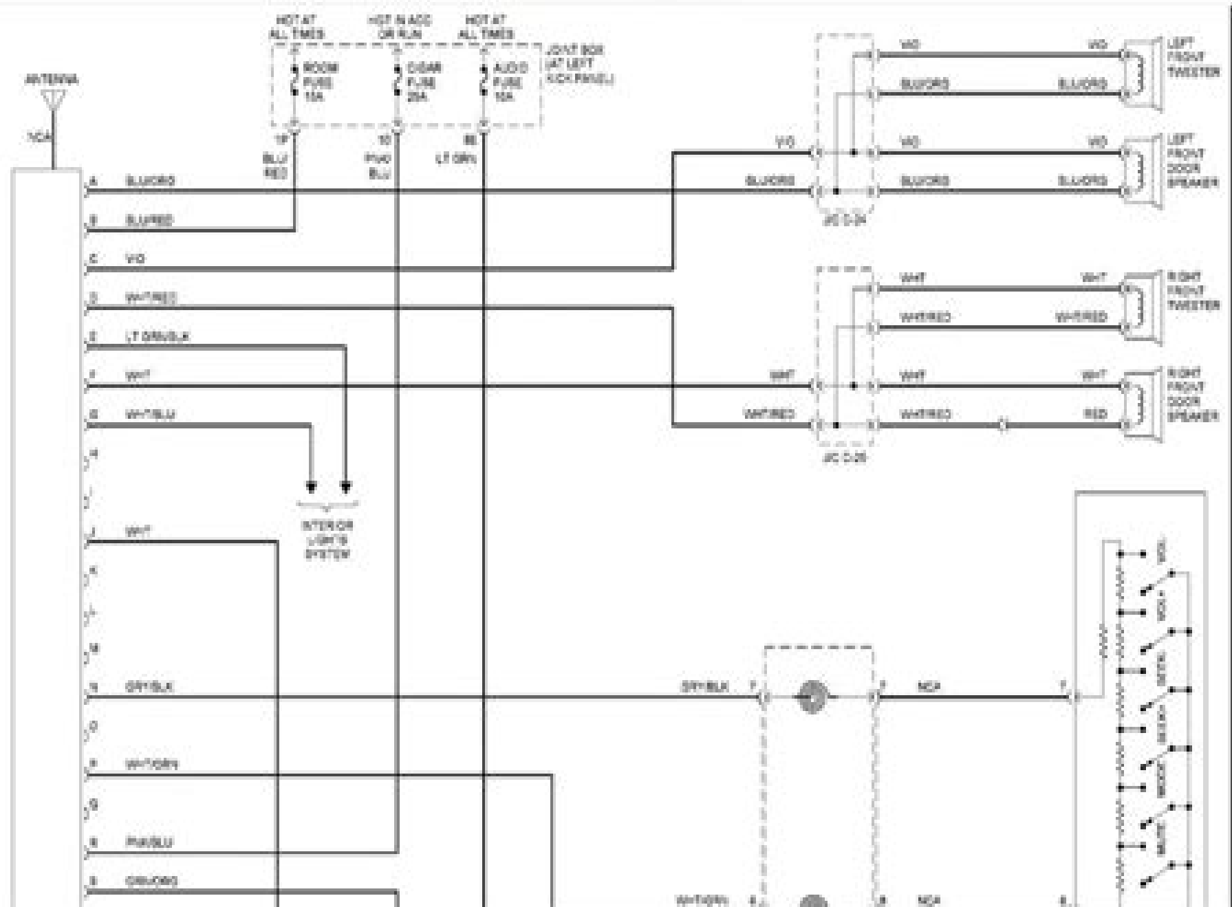
Fig. 32: Radio Circuit
