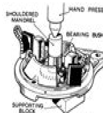
Fig. 20. Method of fitting the armature bearing bush.
