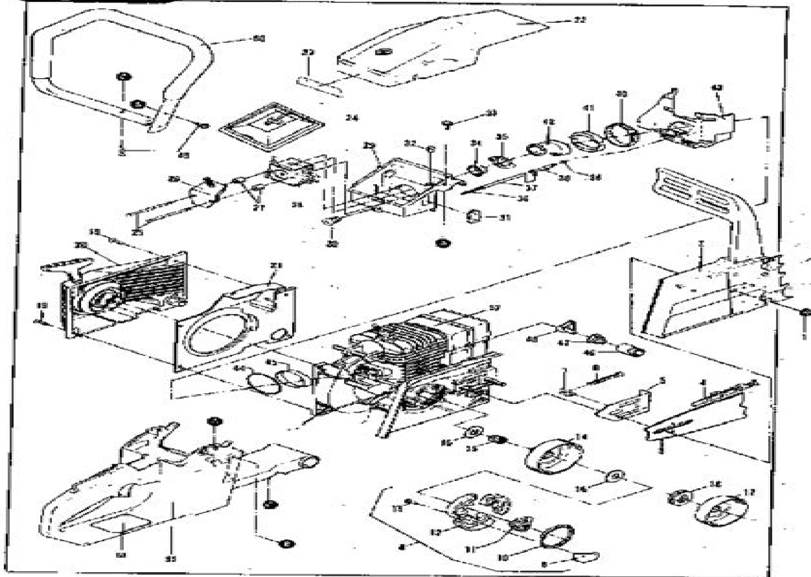
Figure 1 GENERAL ASSEMBLY
