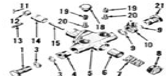
Fig. 62—Exploded view of fuel pump shown in Fig. 61. Hand primer lever is not shown.
