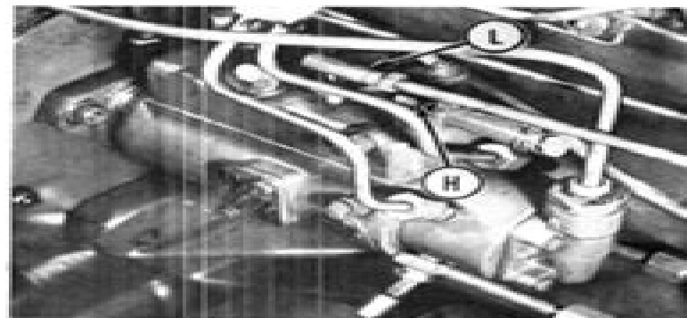
Fig. 60—On late B-275 and all B-414, 354, 364, 384, 424, 444, 2424 and 2444 tractors having injection pump fitted with mechanical governor the high (H) and low (L) idle speed adjusting screws are located as shown.
