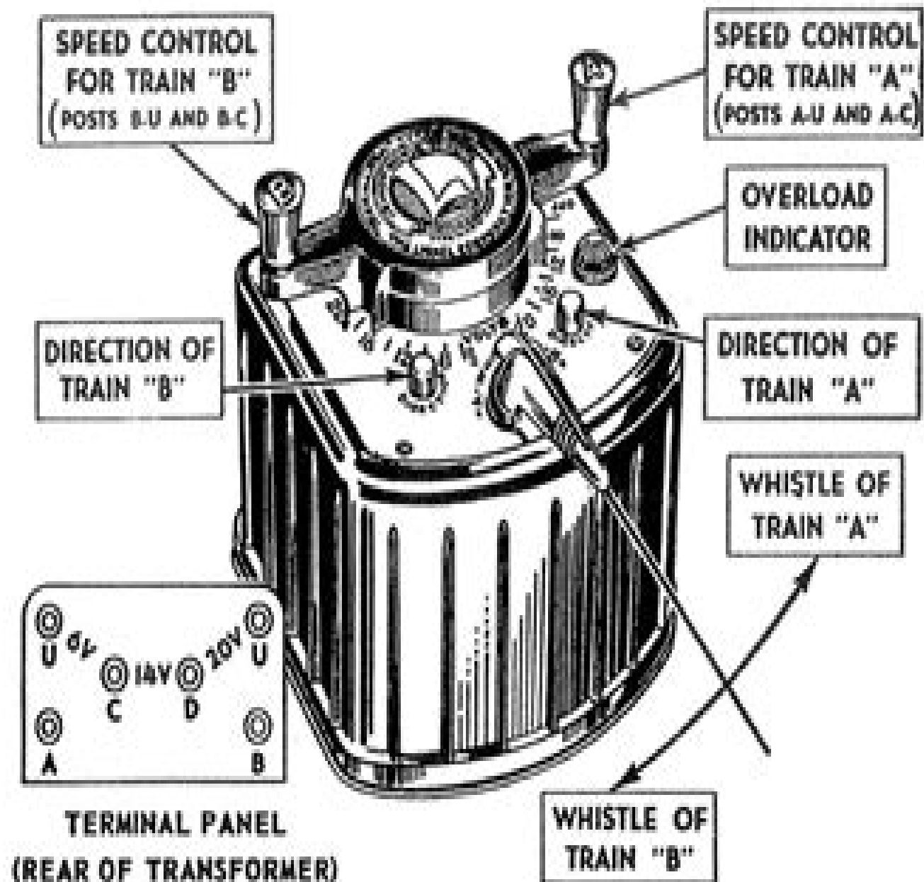
Figure 1—Type "KW" Multi-Control Transformer
