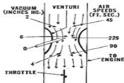
Fig. C55—Schematic view of venturi principle. Right hand figures show how air speed is increased by the restriction (venturi) while left hand figures show the accompanying drop in air pressure.
