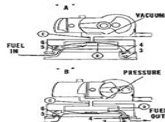
Fig. C57—Schematic view of a typical, crankcase operated, diaphragm type fuel pump. Pressure and vacuum pulsations from crankcase pass through connection (C) to rear of diaphragm (D) which induces a pumping action on fuel flow as shown.
