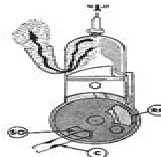
Fig. C53—Two stroke, rotary valve engine. The incoming fuel charge is controlled by a rotary valve effected to the crankshaft. The opening in valve (AO) and crankcase (SO) align at the proper time to admit a fresh charge, then close to allow initial crankcase compression.
