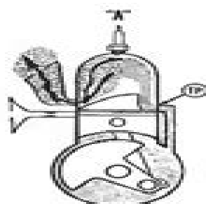
Fig. C52—Two stroke, three port engine. Principles are similar to reed valve or rotary valve types except that a third, intake port is located in cylinder wall and opened and closed by the piston skirt.
