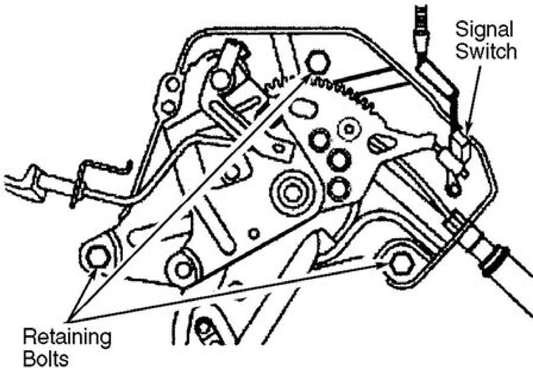
Fig. 18: Locating Park Brake Control Retaining Bolts & Signal Switch
