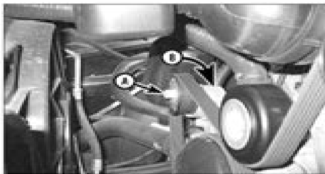
12.5a Place a socket on the tensioner bolt (A) and turn the tensioner clockwise (B) for belt removal
