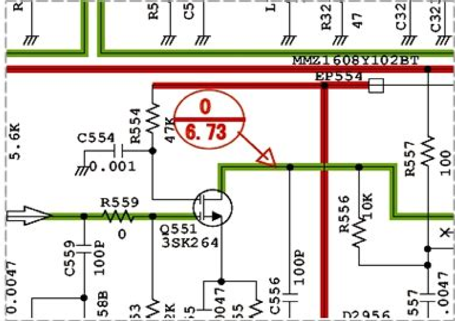
Preview: ICOM IC-7200 schematic diagram
