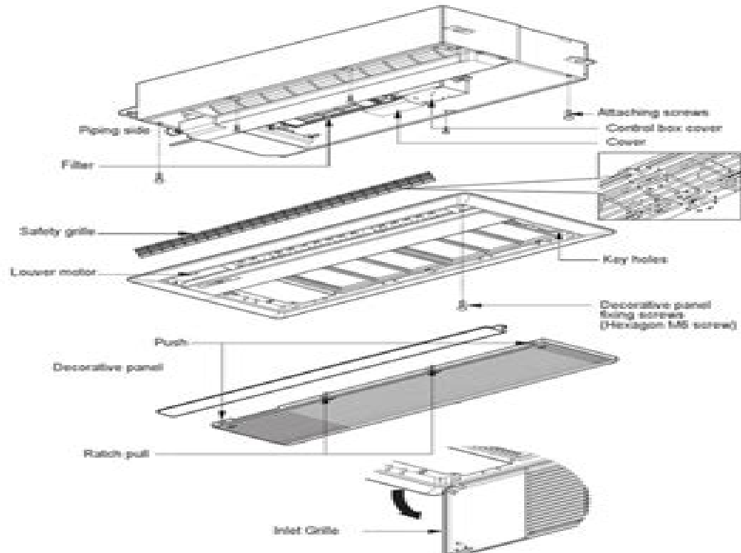
Figure 33: Decoration Panel Installation
