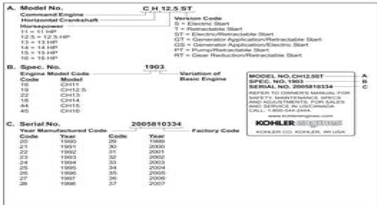
Figure 1-2. Explanation of Engine Identification Numbers.
