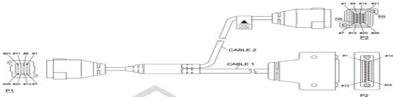
Figure 4-10. J600 Accessory Connector Y-Cable KT000247A01
