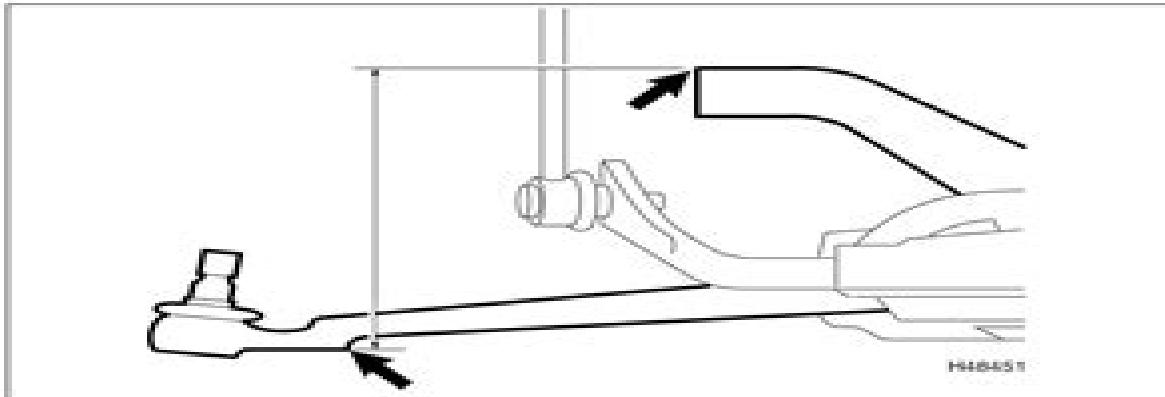
6.16 Raise the lower arm so the distance between the lower edge and the subframe upper edge is 187 mm
