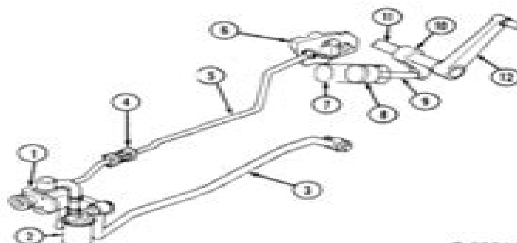
Figure 48 Three-Point Hitch Hydraulic System 1. Hydraulic Pump 2. Hydraulic Inlet Filter 3. Inlet Line 4. Tube Connector 5. Pressure Line 6. Control Valve 7. Lift Cylinder 8. Lift Piston 9. Piston Rod 10. Ram Arm 11. Cross Shaft 12. Lift Arm
