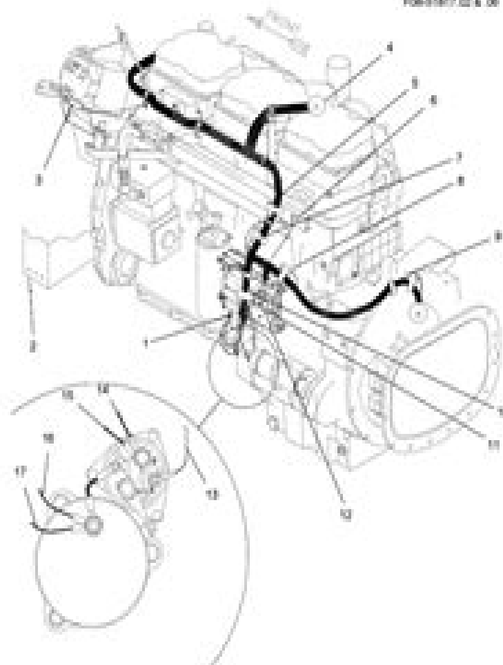
Figure 22 Engine Wiring, C-10 & C-12
