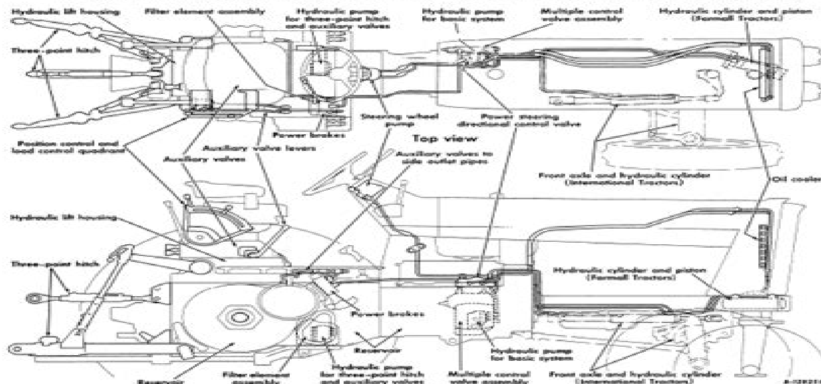
Illustr. 25 Hydraulic systems diagram.
