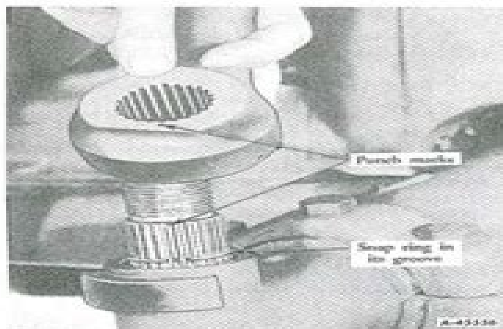
Illustr. 22. Punch marks on land and groove must be aligned when assembling steering knuckle arm.
