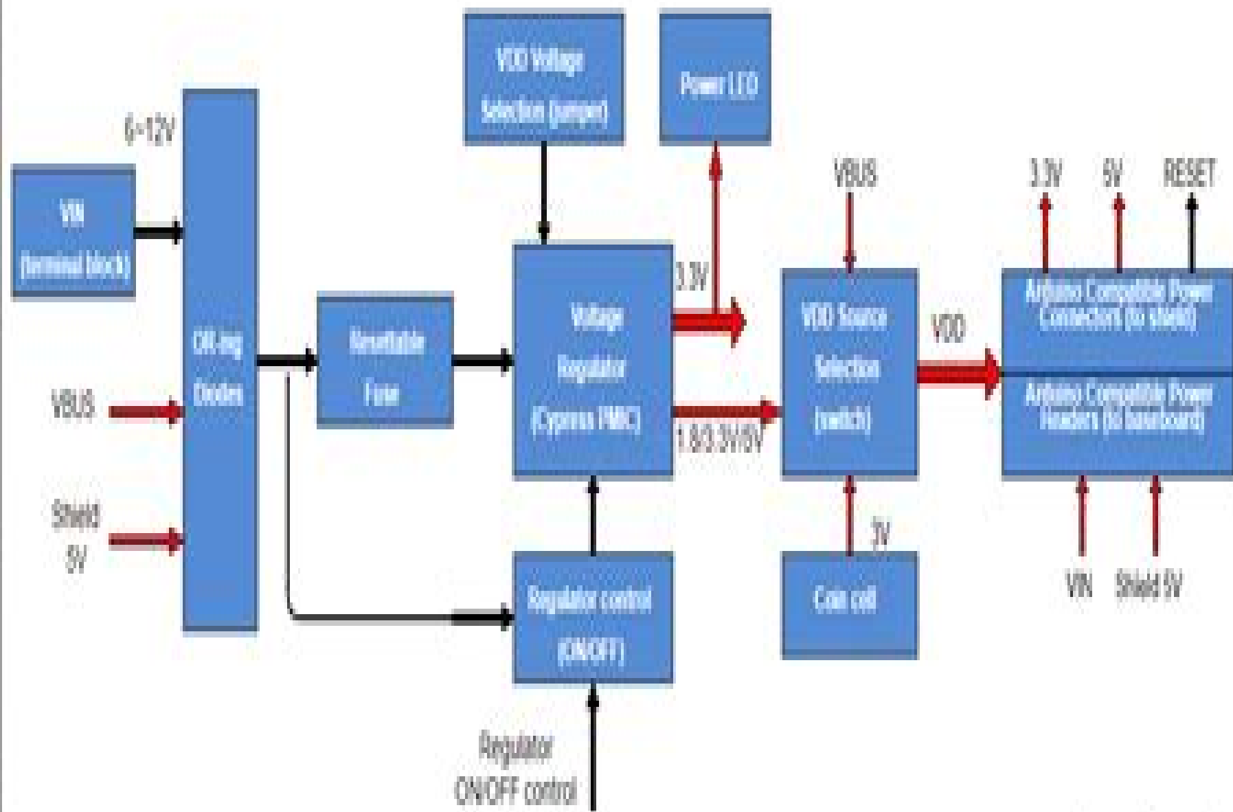
Power Supply
