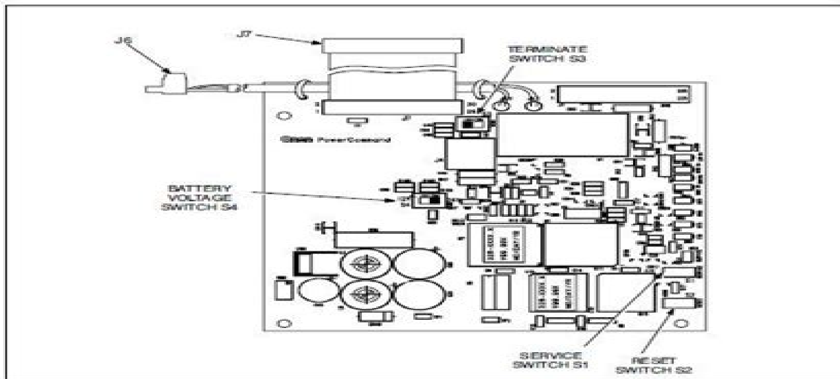
FIGURE 3-10. GENSET COMMUNICATIONS MODULE
