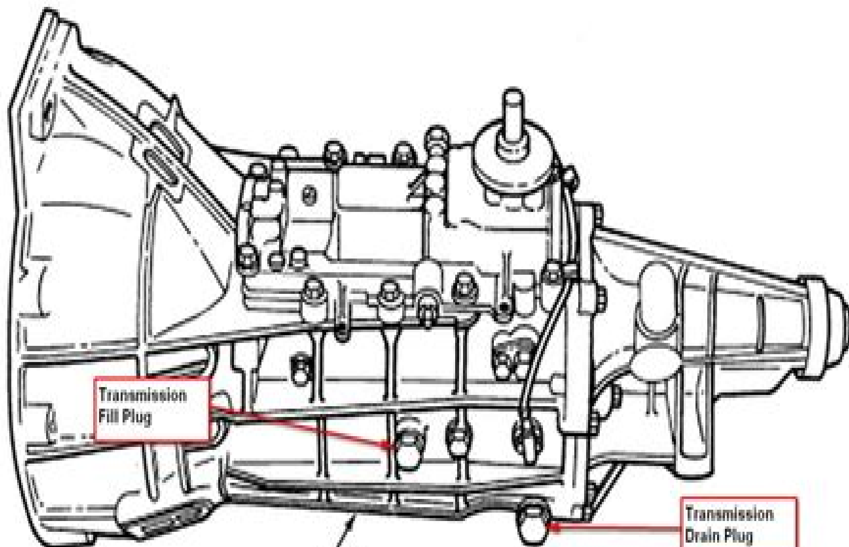
M50D TRANSMISSION ASSEMBLY
