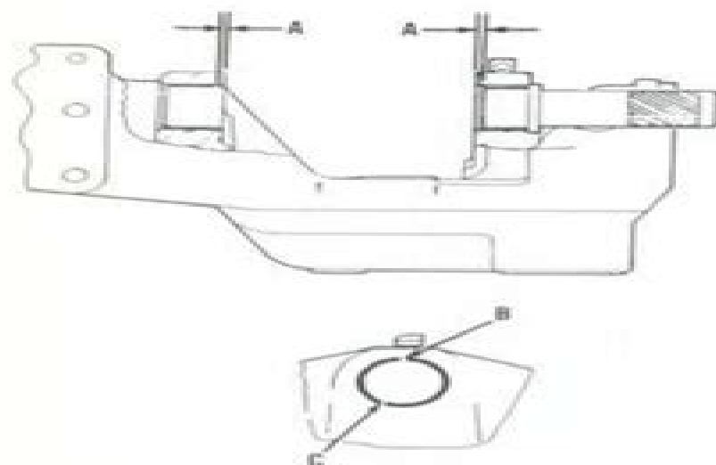
Fig. 9—Axle pivot bushings should be installed as shown for 362 model. Hole (B) should be aligned with grease passage and slot (C) should be in position indicated.
