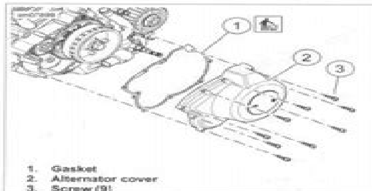
Figure 4-33. Alternator Cover
