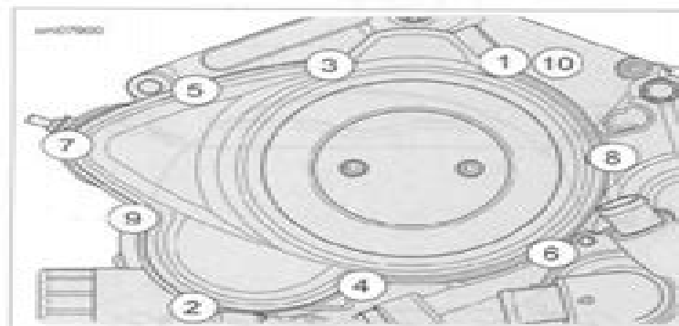
Figure 4-34. Tightening Sequence
