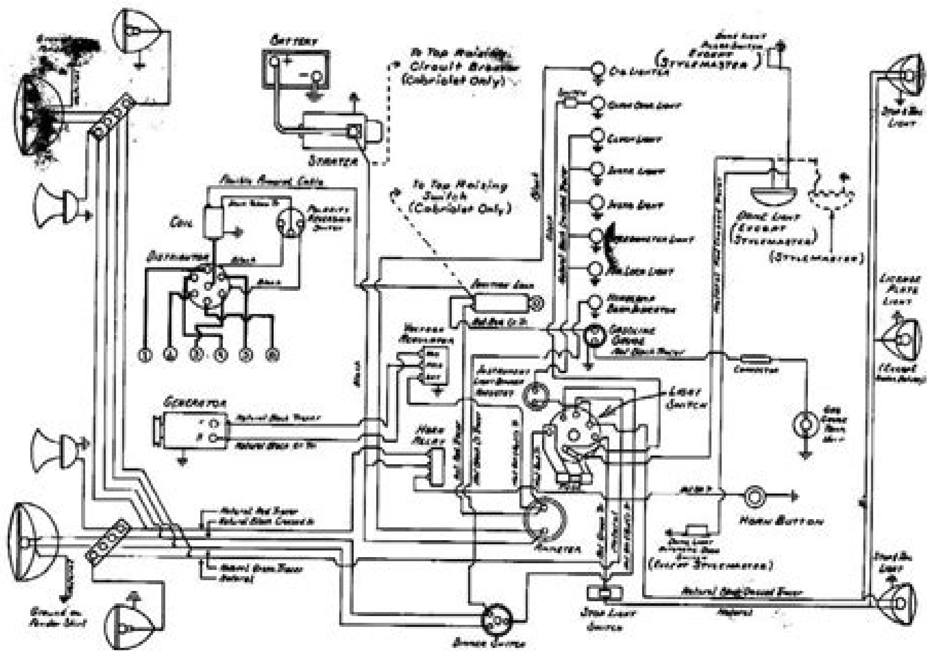
Fig. 65—Passenger Car Wiring Diagram
