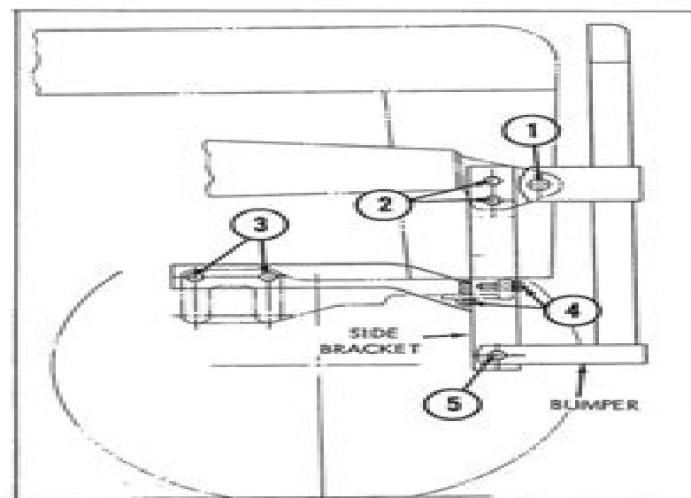
Fig. 9 - Mounting Kit Installation - MF 50 (F 40 & MH 50) and MF 65 Tractors
