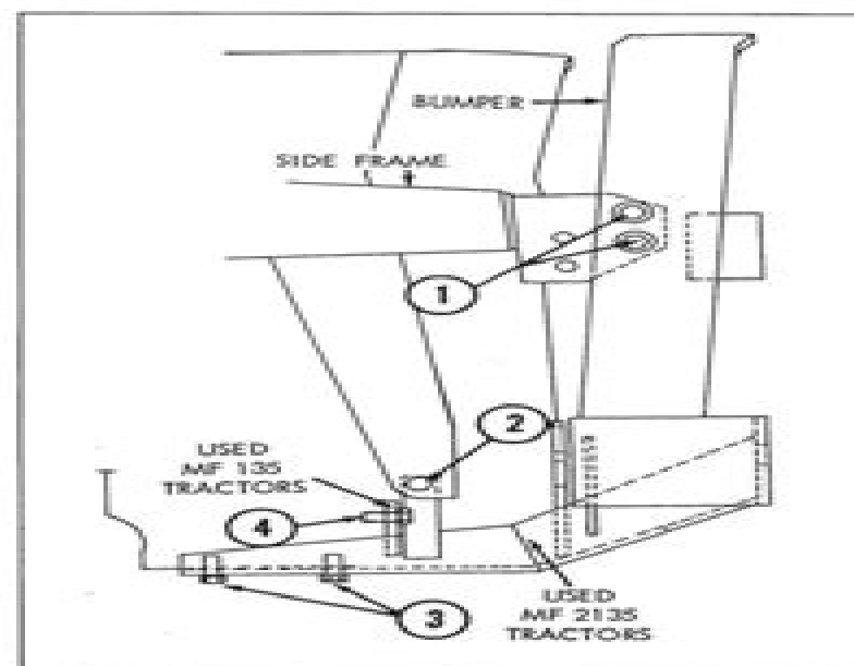
Fig. 10 - Bumper Installation - Used on MF 135 and MF 2135 Tractors
