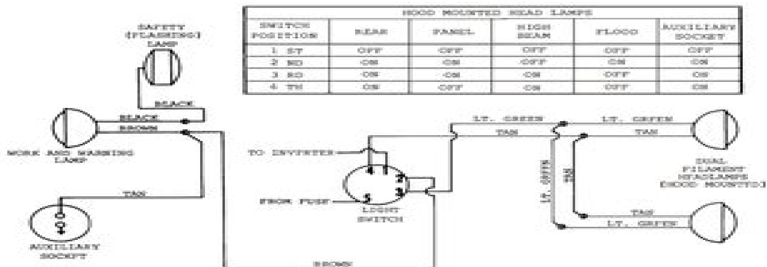
Fig. 81 - Electrical System - Hood Mounted Headlamps
