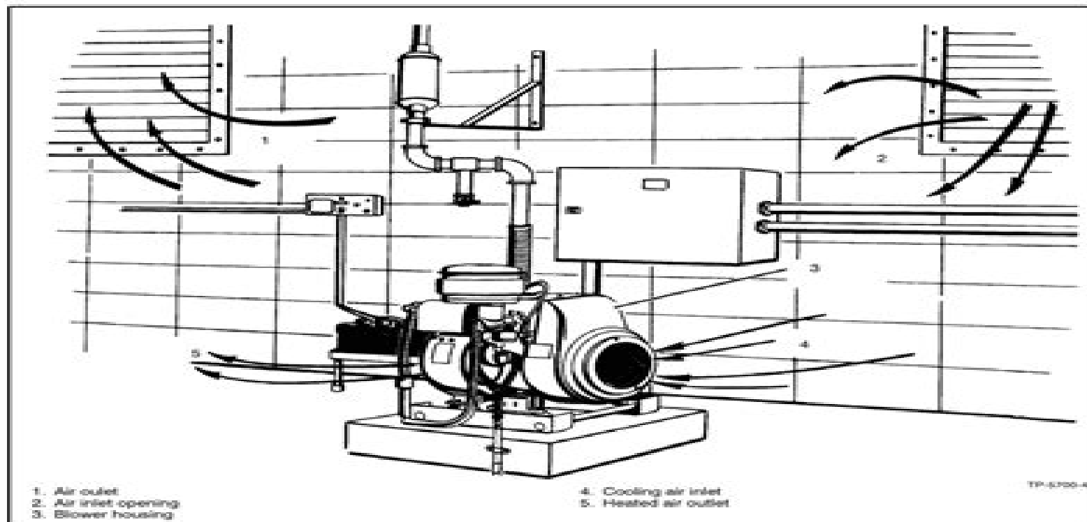
Figure 4-5 Standard Forced-Air Cooling System
