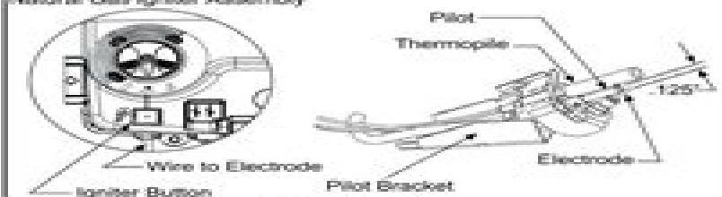
Figure 29 Natural Gas Igniter Assembly
