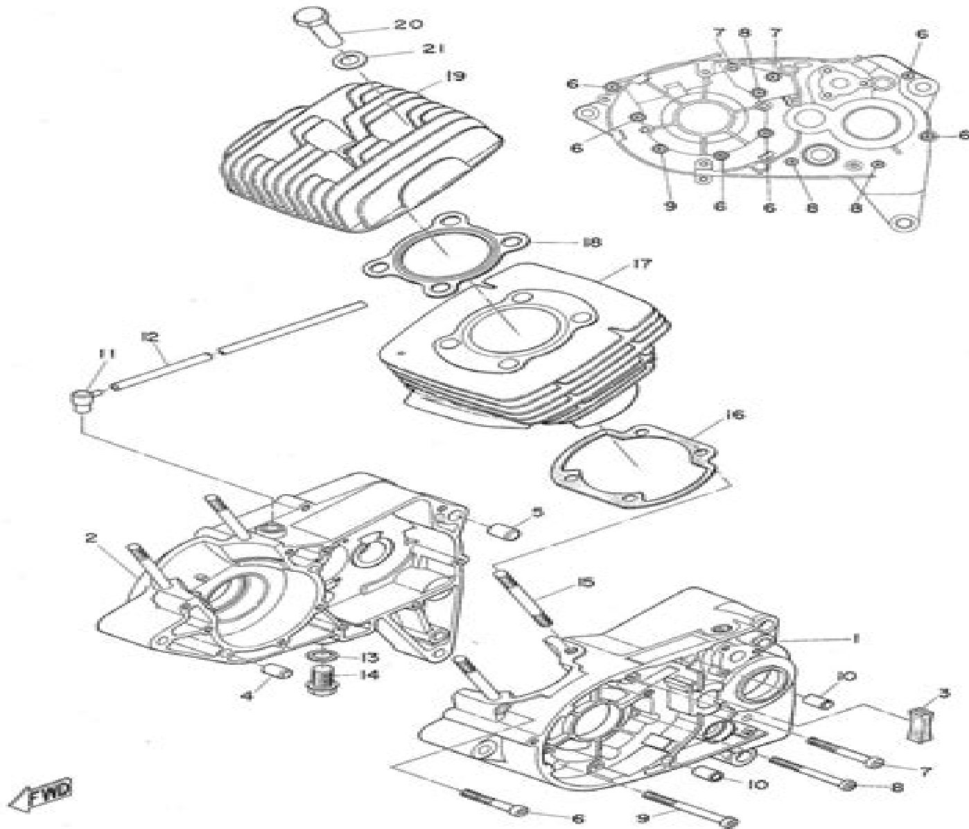
Fig. 1 CRANKCASE
