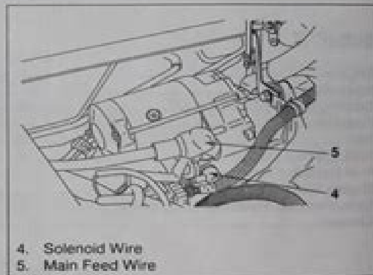
Figure 2. Wiring at Starter
